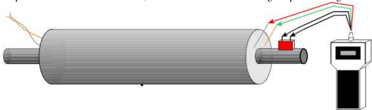
Fig. 1. LX-9024 connection diagram
